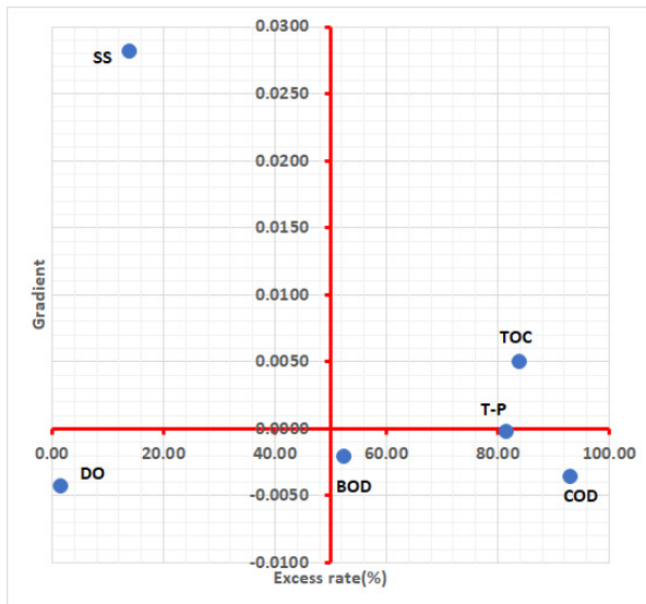
(a) DO, BOD, COD, SS, T-P, TOC
