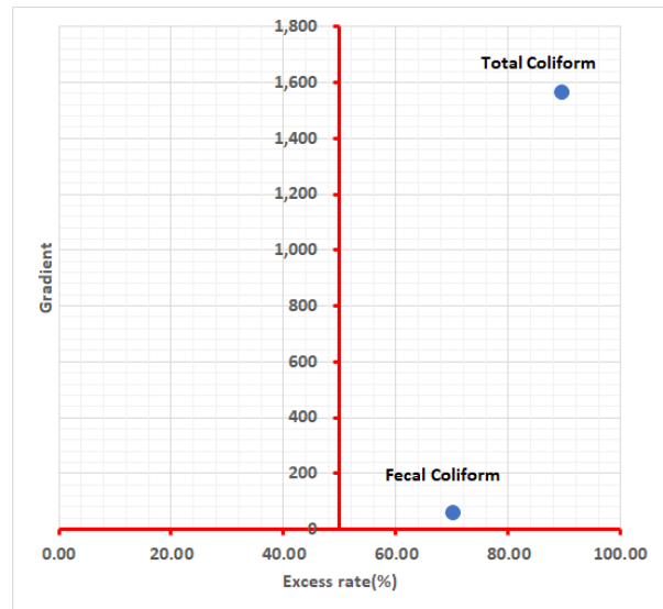
(b) Fecal Coliform, Total Coliform
