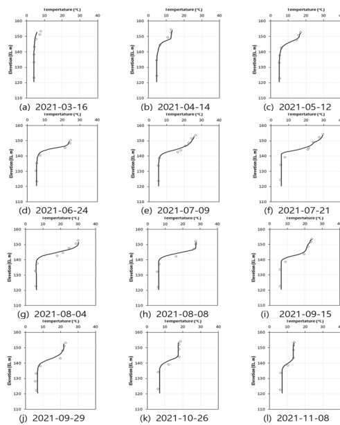
Fig. 6. Model calibration results for thermal stratification reproducibility in 2021
