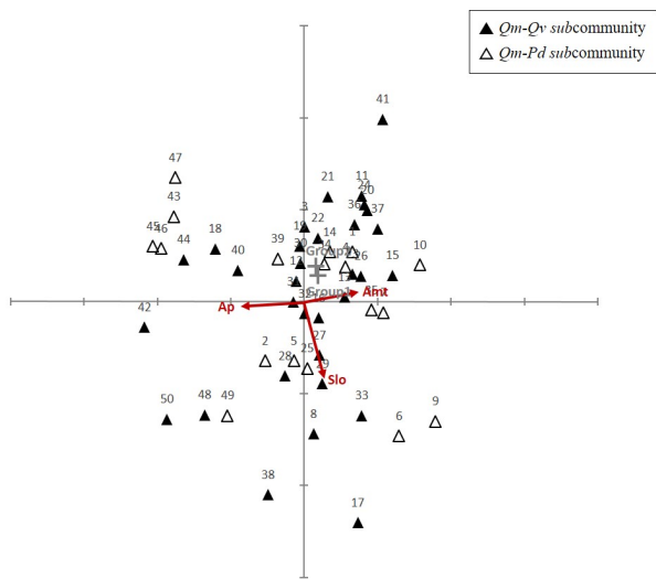
Fig. 3. CCA ordination biplot of importance value and 5 environmental variables in 50 stands which are classified by plant community. The community classification are ▲: Quercus mongolica - Quercus variabilis subcommunity, △: Quercus mongolica - Pinus densiflora subcommunity. The arrows on graph mean significant environmental variables which are influencing on stands, the environmental variables are Annual precipitation(Ap), Slope(Slo), Annual mean temperature(Amt) and cross shape shows centroids of each group.
