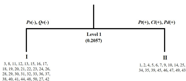
Fig. 2. Stand classification by TWINSpan using the importance value of species of Quercus mongolica community in the central region of Korea, the number for each group indicates the stand that corresponds to each group (Qv: Quercus variabilis , Ps: Prunus sargentii , Pt: Parthenocissus tricuspidata , Cl: Carex lanceolata , Pd: Pinus densiflora )
