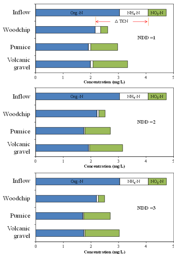
Fig. 10. Comparison of the nitrogen conversion among the three wetland beds
